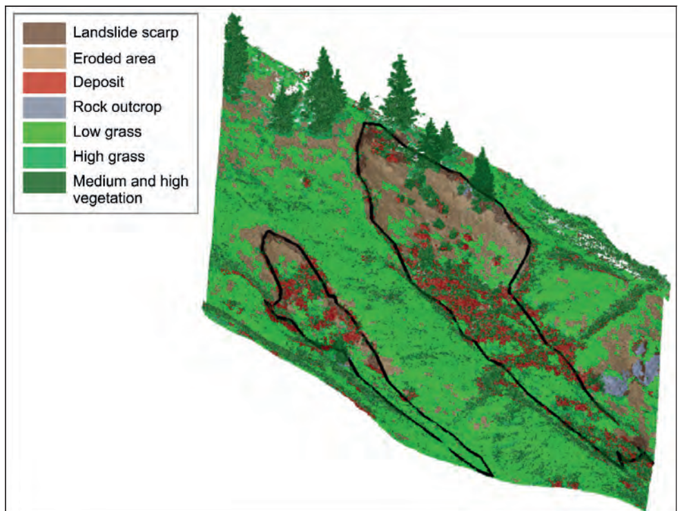
▲ Figure 3: Random forest classification of a point cloud and reconstructed landslide shapes (black).
