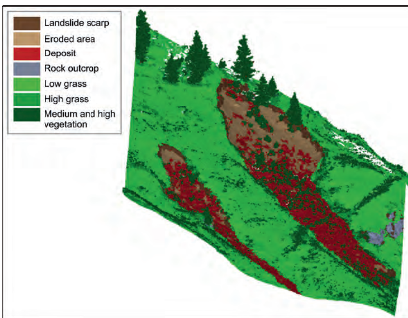
▲ Figure 4: Final classification result.
