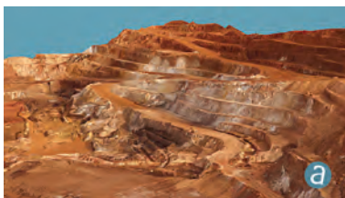
Correlator3D 8.0.
