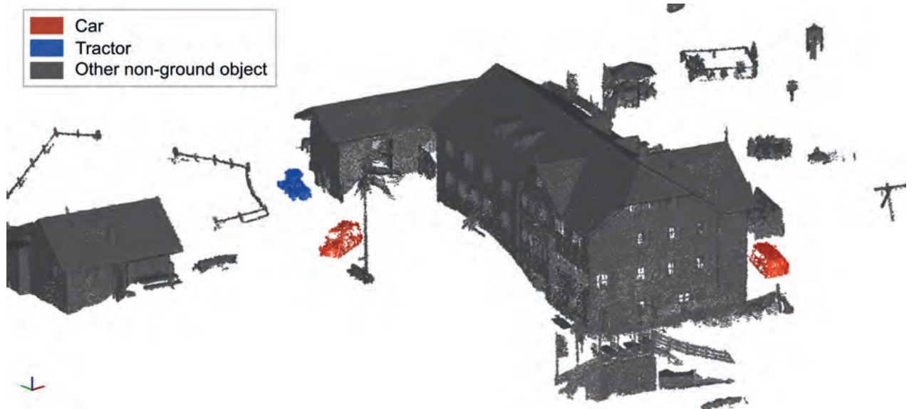
▲ Figure 1: Subset of a classified point cloud from a Lidar UAV.
