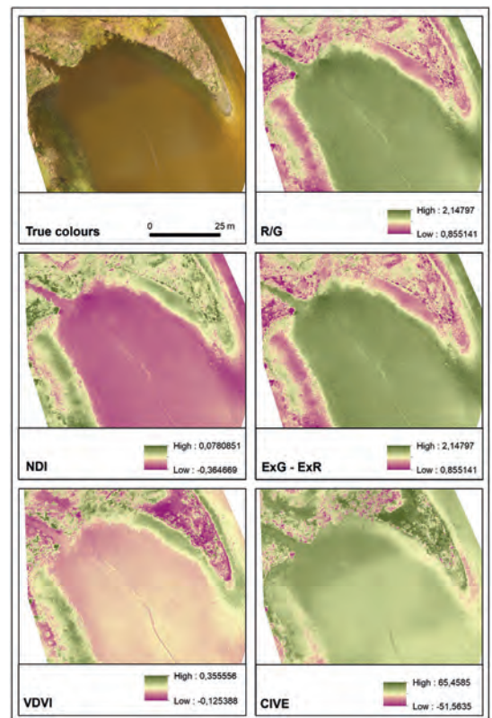
▲ Figure 2: Area of interest and calculated vegetation indices.
