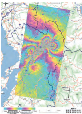
Crustal deformation analysis by InSAR.
