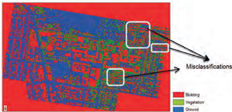
▲ Figure 3: Building classification of 2005 Lidar data using SVM.
